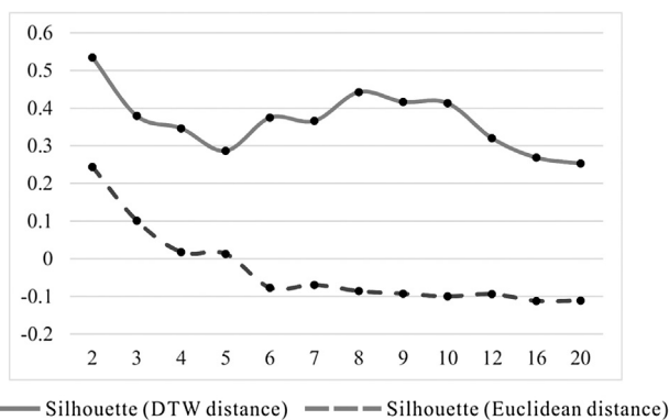
Fig. 4. The silhouette metric values of different experimental results (y axis) by varying the number of clusters k (x axis).
